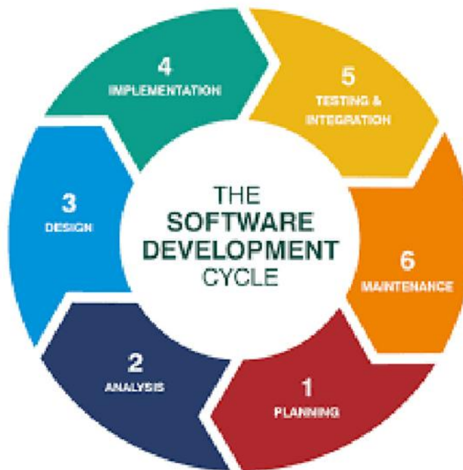
Figure 1:SDLC Model
