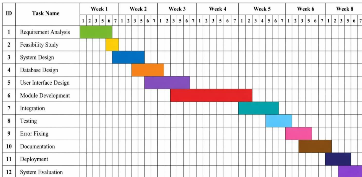
Figure 2: Gantt Chart
